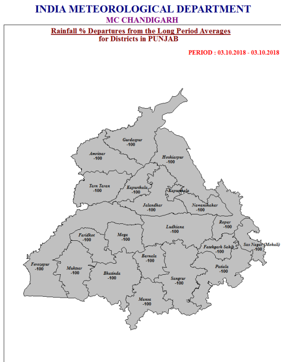
Figure 1: District wise Daily Rainfall Departure.
